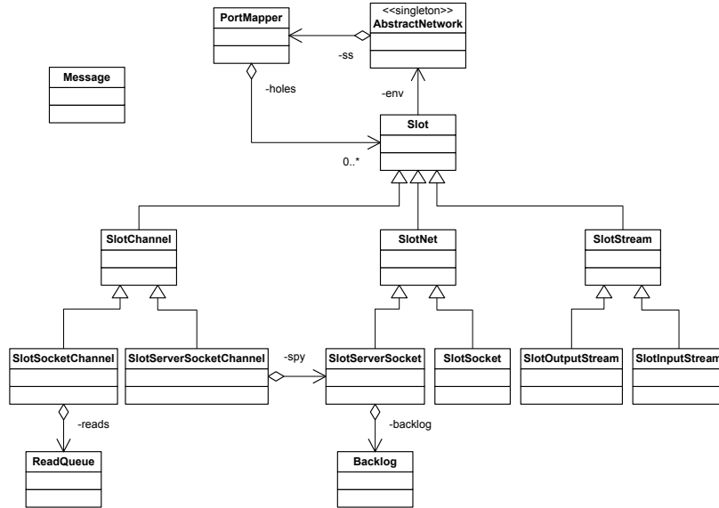
Fig. 5. The Abstract Network class hierarchy
