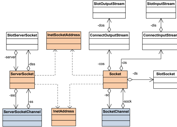
Fig. 4. MJJ model for the Socket API
